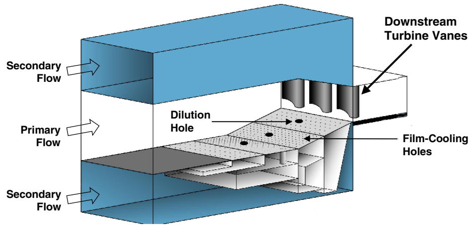
Combustor Simulator
